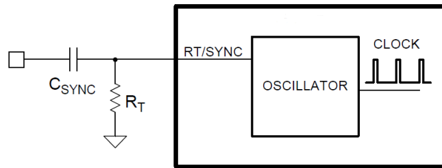
Figure 2. Oscillator Synchronization through AC Coupling
