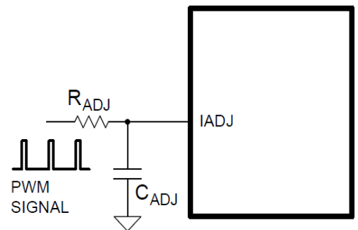
Figure 6. Analog Dimming Achieved By Low-pass Filtering External PWM Signal
