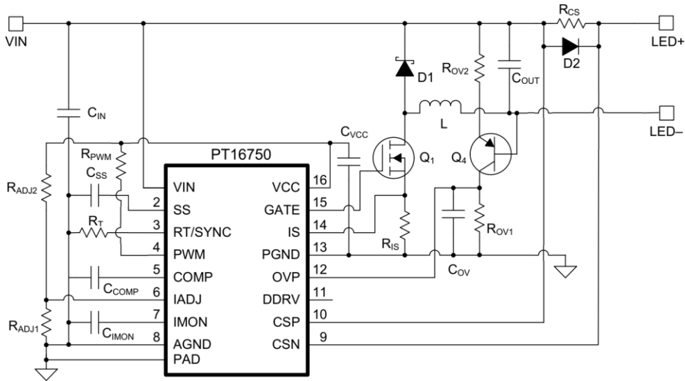
Figure 12. Buck LED Driver
