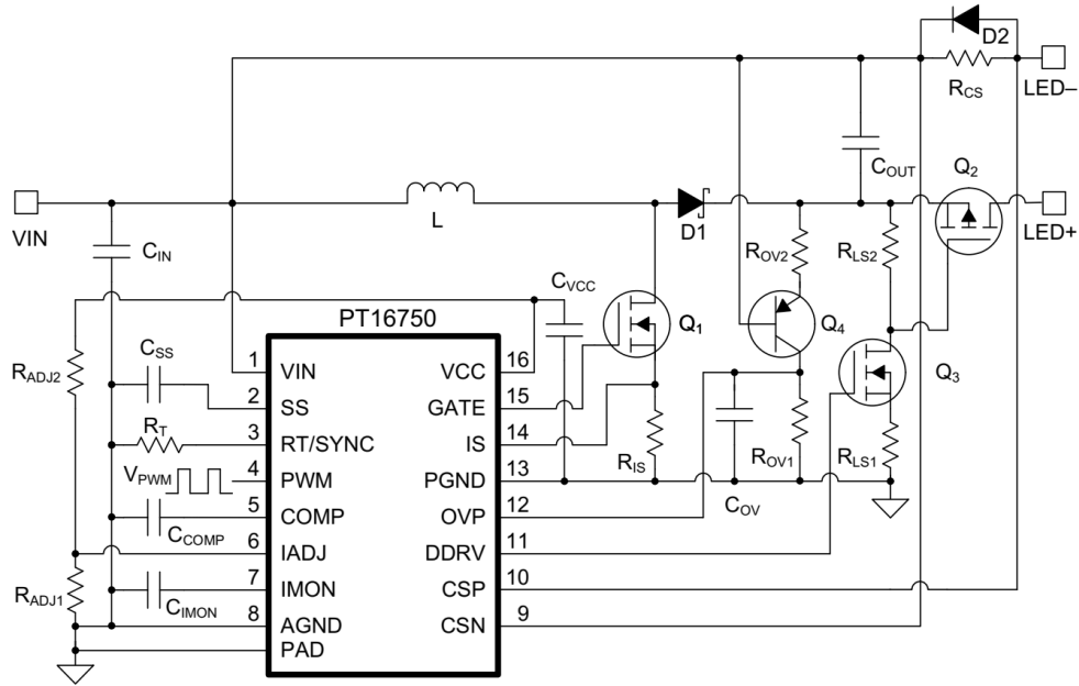
Figure 11. Buck-Boost LED Driver
