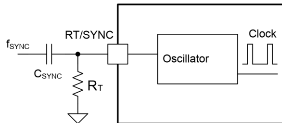
Figure 2. Oscillator Synchronization Configuration
