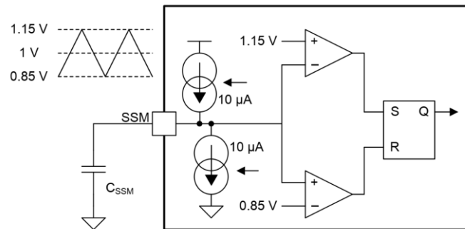
Figure 3. Spread Spectrum Modulation
