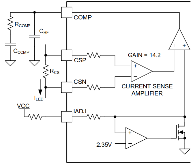
Figure 26. Proportional-Integral Compensation
