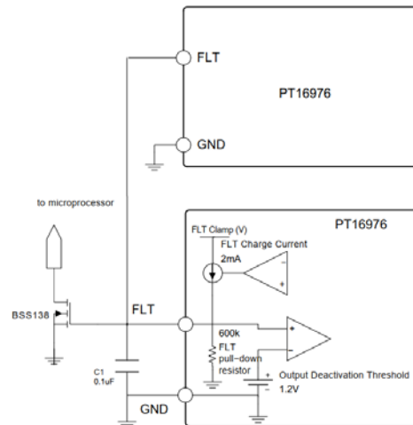
Figure 5. Multiple IC implementation of Open Load Detection
