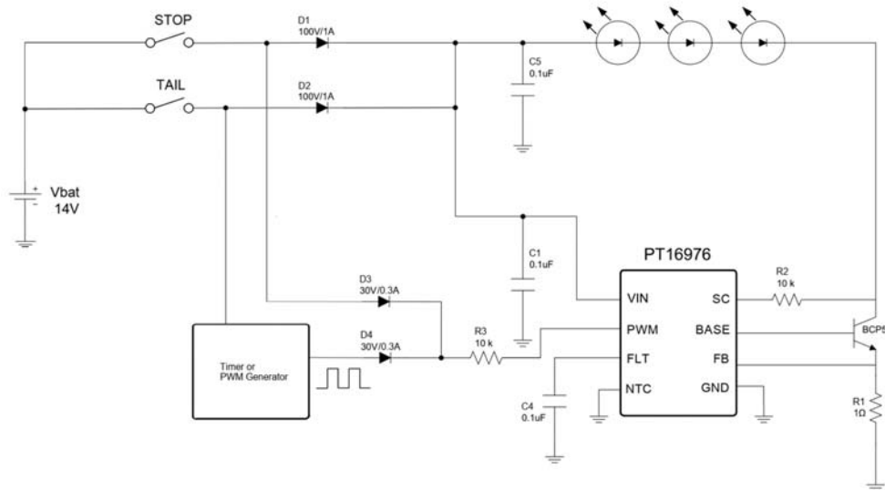
Figure 11. Stoplight / Taillight Application
