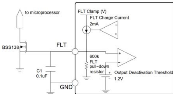
Figure 4. FLT Output Interface to Microprocessor
