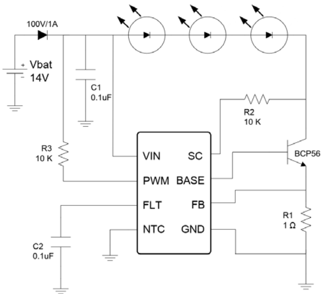
Figure 12. Application Diagram with No Microprocessor
