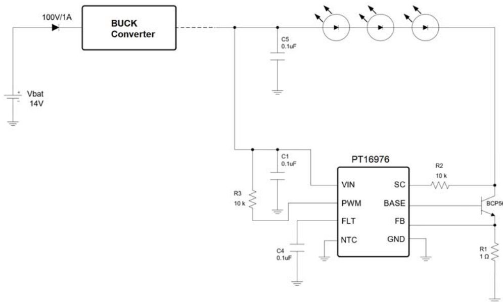
Figure 10. High Efficiency Application
