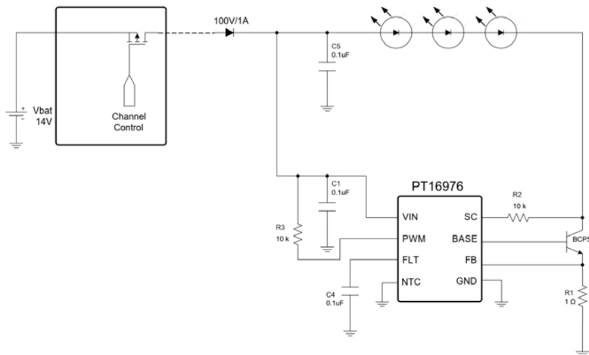
Figure 9. External Power-on control
