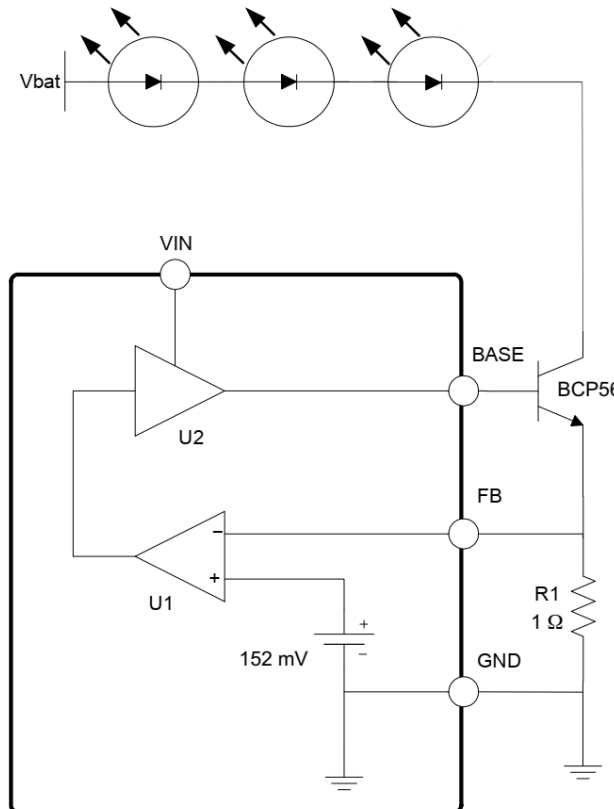
Figure 1. Output Drive Configuration
