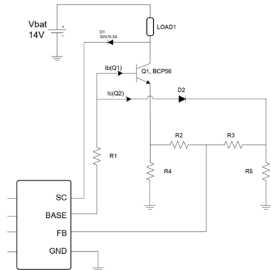
Figure 15. Open Circuit Equivalent
