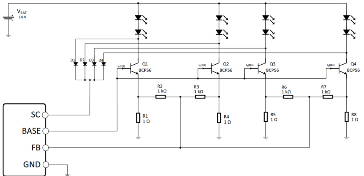
Figure 8. Short Circuit Detection with 4 or more Channels
