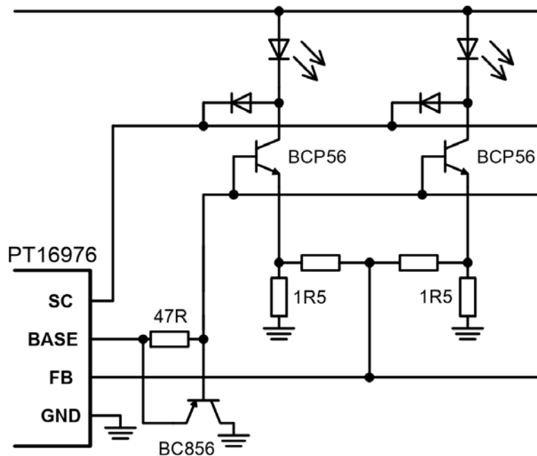
Figure 3. Improved Open Load Detection for Multiple Strings
