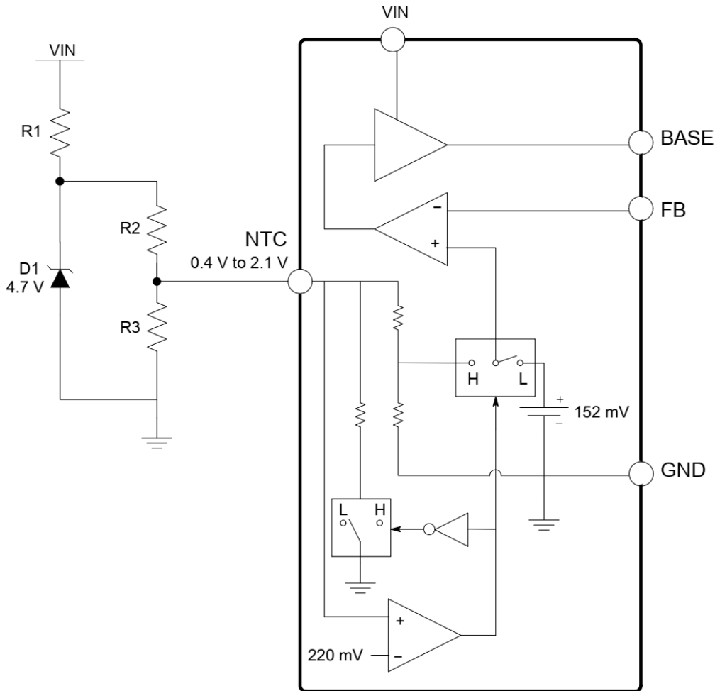
Figure 6. Negative Temperature Compensation Operation
