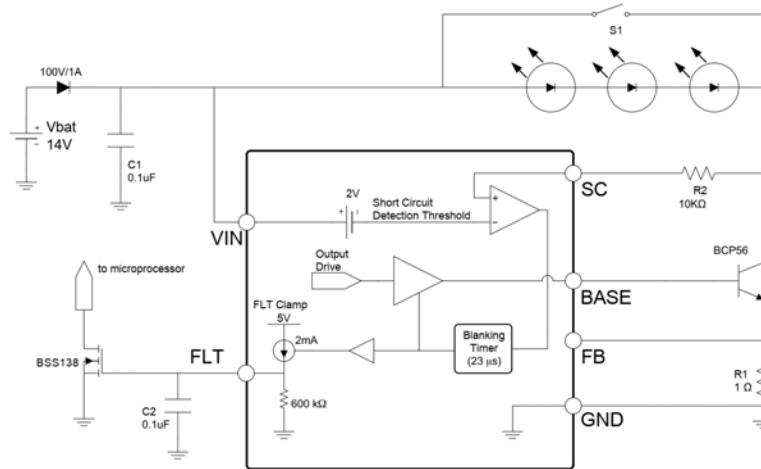
Figure 7. Short Circuit Detection
