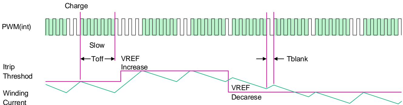
Figure 2. PWM Current Regulation Operation Period and Timing
