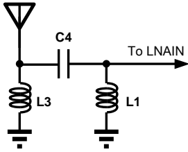
Figure 11. Antenna ESD Protection Inductor of PT4301
