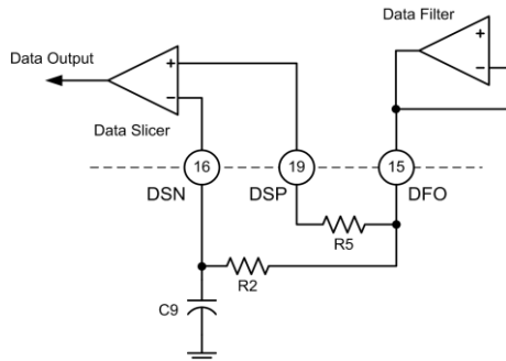
Figure 8. Circuit for Generating Data Slicer Threshold
