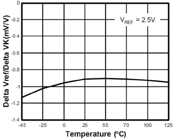
Delta Reference Voltage vs. Temperature
