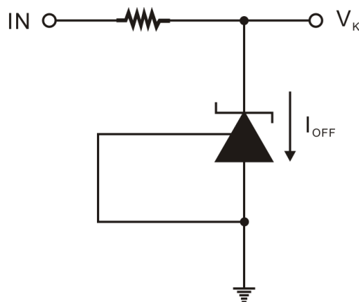
Figure 3. Off-State Current
